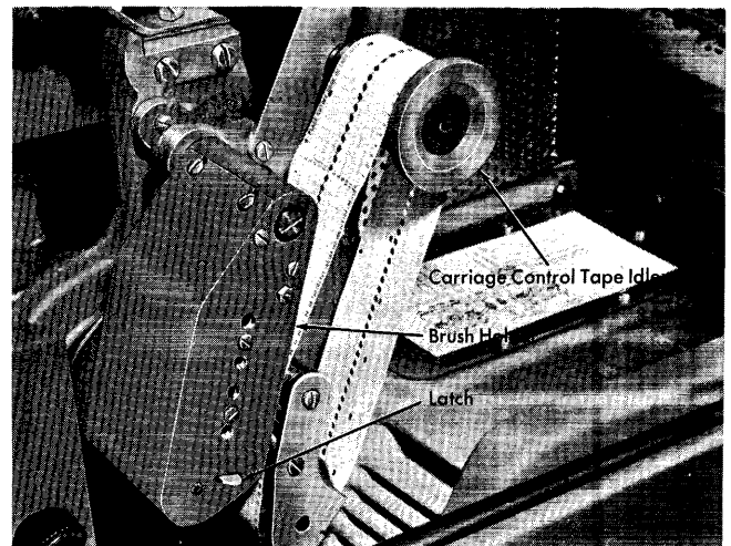
Figure 205. Tape-Controlled Carriage
