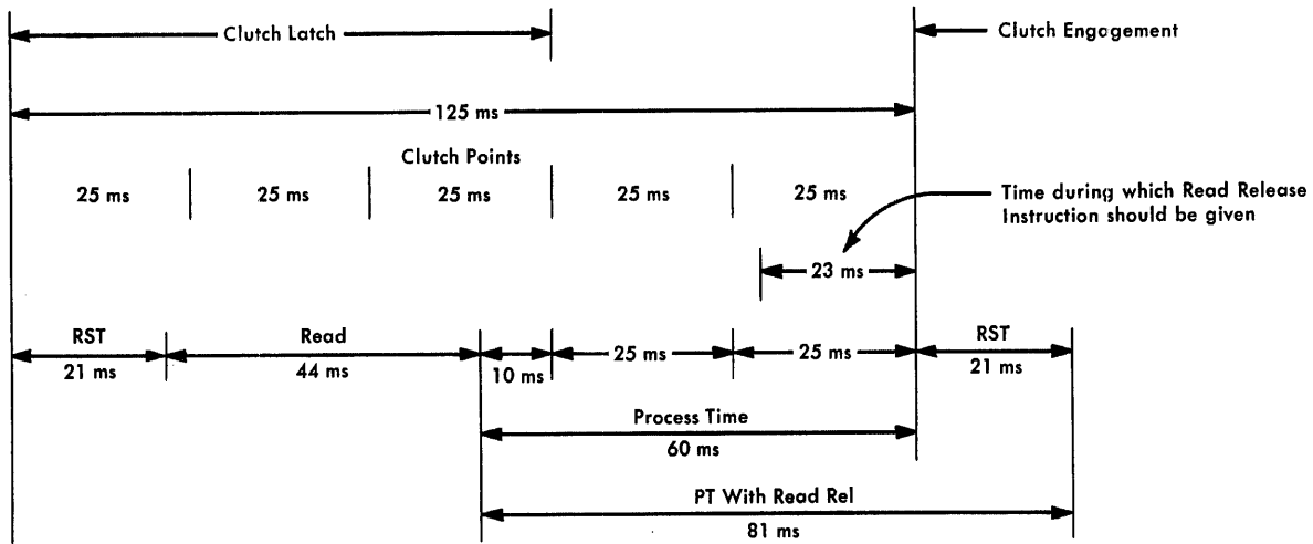
Figure 226. 480 CPM with Early Card Read
