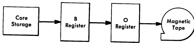
Figure 176. Overlapped Write Magnetic-Tape Operation
