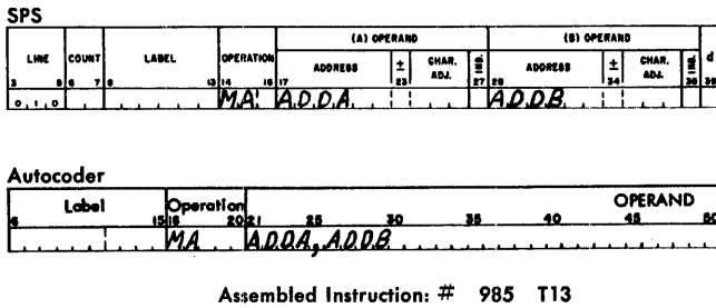
Figure 139. Modify Address (Two-Address)
