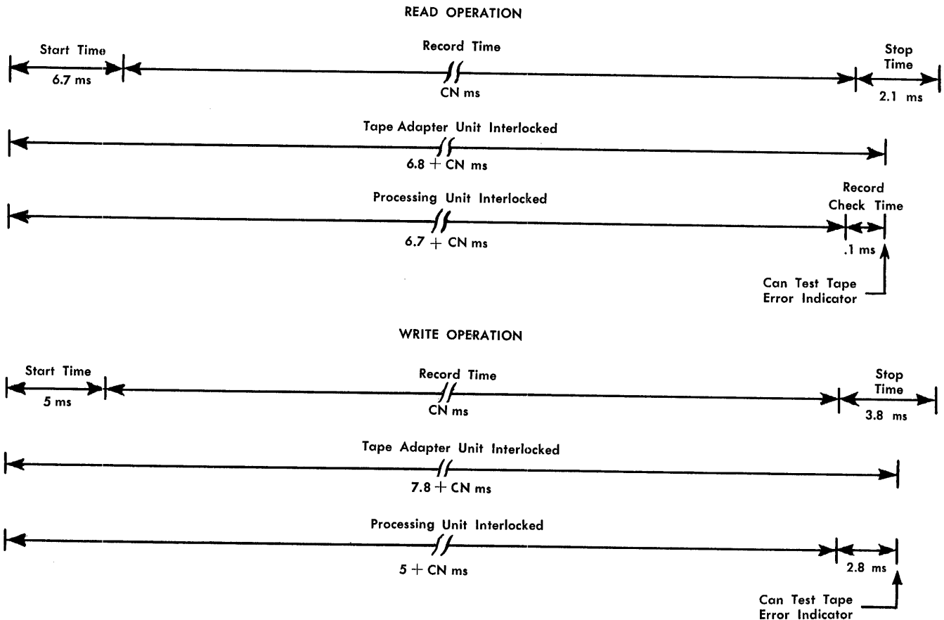
Figure 246. IBM 729, Model IV, Read-Write Tape Timing
