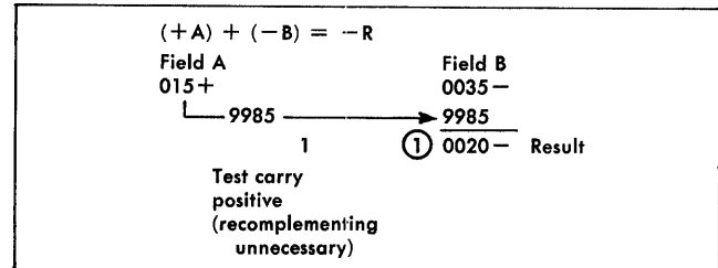
Figure 25. Complement Add with No Recomplementing
